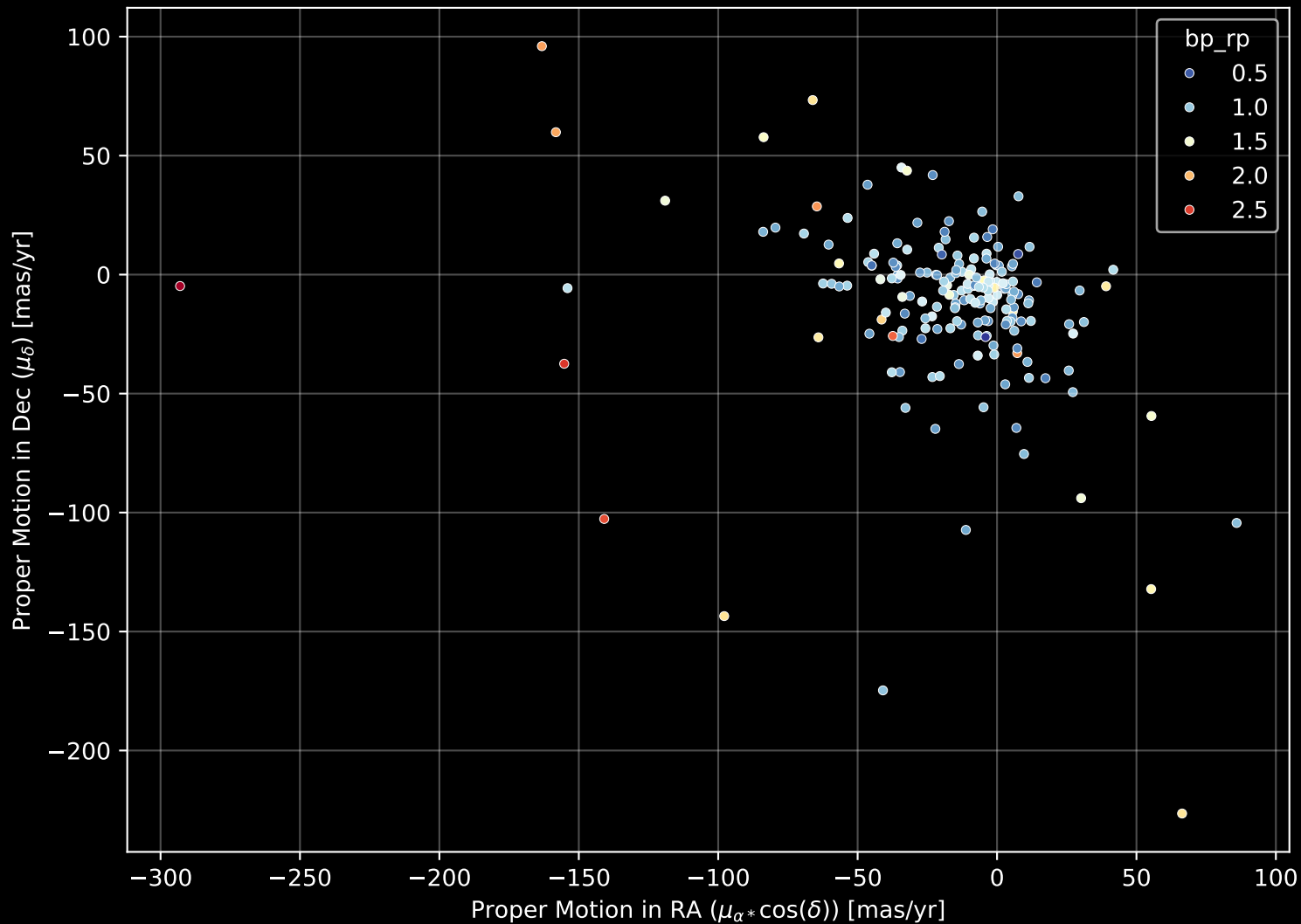
APOGEE DR17 Field: [030+79_MGA] Proper Motion Diagram (n= 191)
