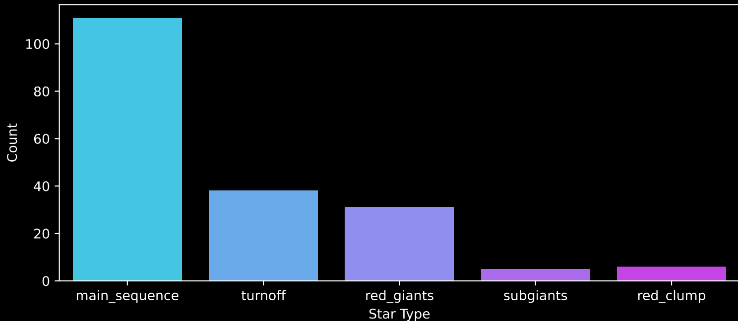
APOGEE DR17 Field: [030+79_MGA] Count plot of Star Type
