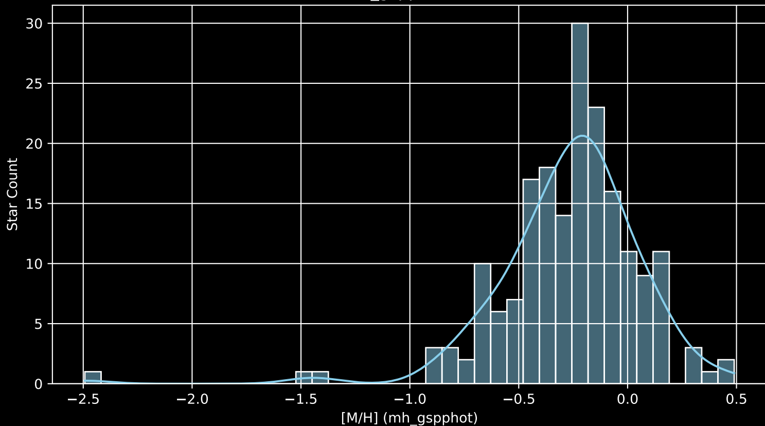
APOGEE DR17 Field: [030+79_MGA [M/H] (mh_gspphot) (n= 189)
