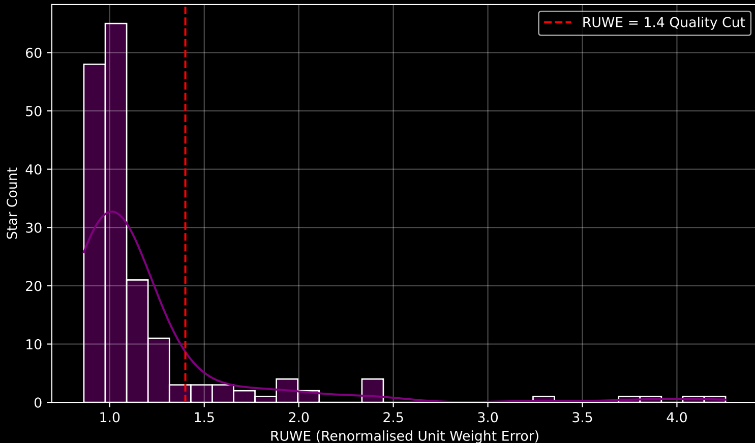
GAPOGEE DR17 Field [030+79_MGA] RUWE Distribution (n= 182)
