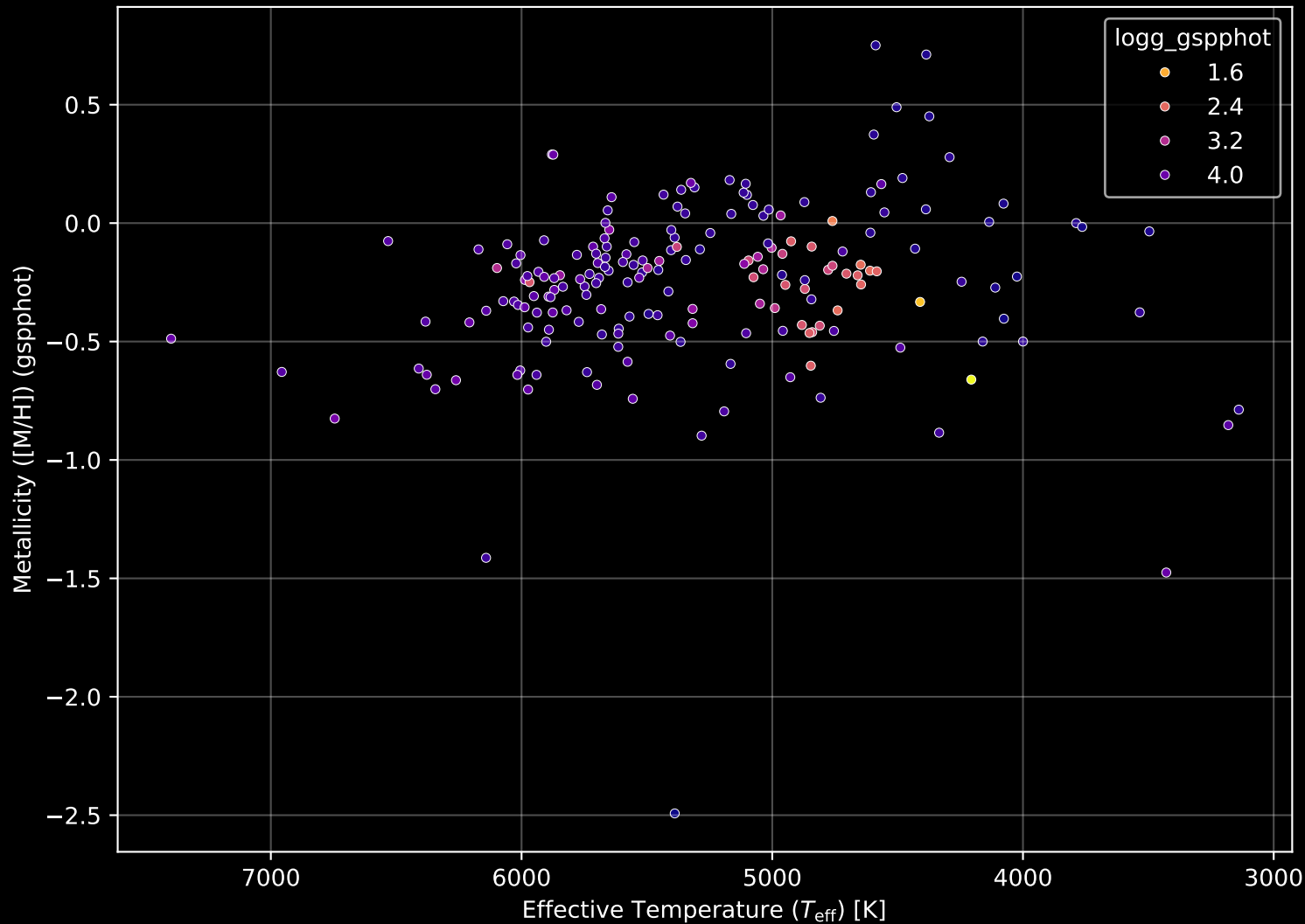
APOGEE DR17 Field: [030+79_MGA] Stellar Population Parameters (n= 191)
