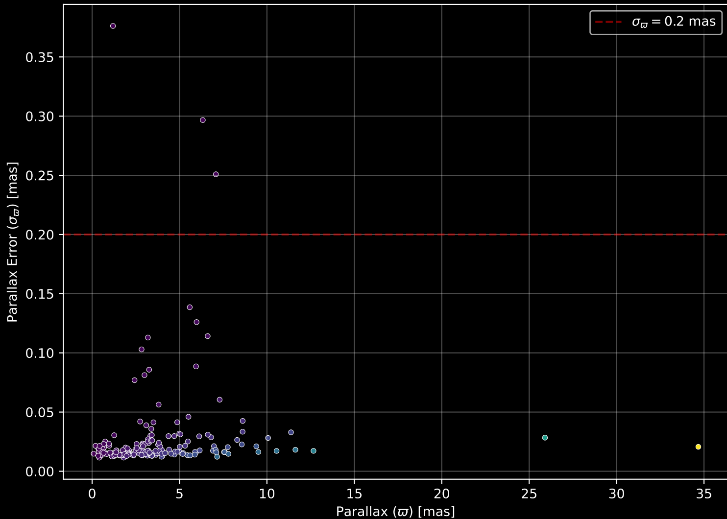
APOGEE DR17 Field: [030+79_MGA] Parallax Quality (n= 191)
